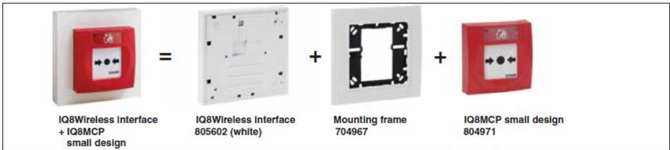
Mounting IQ8Wireless interface with IQ8MCP small design
